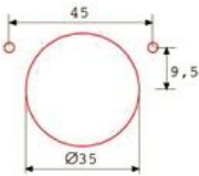
For hinges type "Salice"
