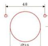
For hinges type "Hattich"
