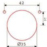
For hinges type "Blum"
