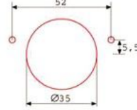
For hinges type "Hafele"
