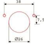
For hinges type "Grass"
